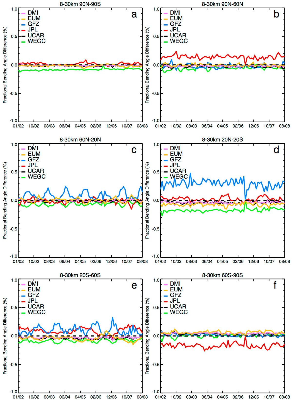
Figure 8. The time series of fractional bending angle differences among six centers for the 8 km to 30 km layer is shown for all investigated zones: (a) the entire globe ( 90^{\circ}\text{N} to 90^{\circ}\text{S} ), (b) 90^{\circ}\text{N} to 60^{\circ}\text{N} , (c) 60^{\circ}\text{N} to 20^{\circ}\text{N} , (d) 20^{\circ}\text{N} to 20^{\circ}\text{S} , (e) 20^{\circ}\text{S} to 60^{\circ}\text{S} , and (f) 60^{\circ}\text{S} to 90^{\circ}\text{S} . The inter-model mean was subtracted on a monthly basis.
