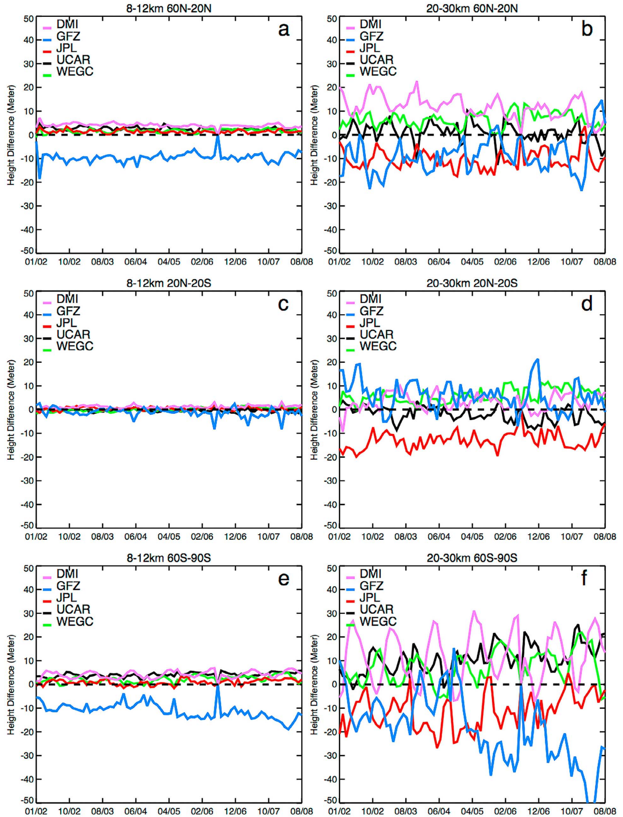
Figure 12. The time series of geopotential height differences among five centers are shown for the 8 km to 12 km layer for (a) the 60°N to 20°N zone, (c) the 20°N to 20°S zone, and (e) the 60°S to 90°S zone, and for the 20 km to 30 km layer for (b) the 60°N to 20°N zone, (d) the 20°N to 20°S zone, and (f) the 60°S to 90°S zone.
